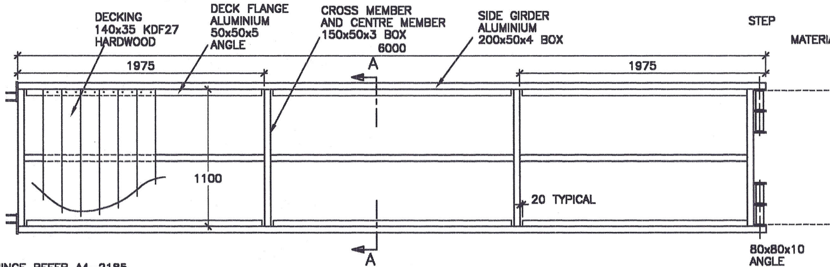
PLAN VIEW
